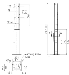
Drawing 1 MB 560
