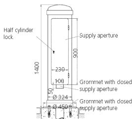
Drawing 1 MB 445 Dim. in mm
