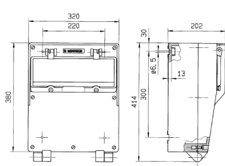
Drawing 5 MB 41
