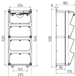
Drawing 1 MB 523
